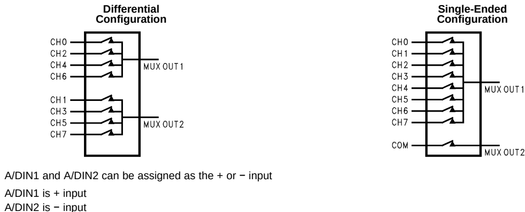
Figure 68. MUXOUT connections for multiplexer option
